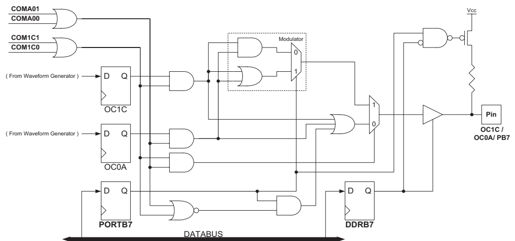
Figure 19-2. Output Compare Modulator, Schematic
