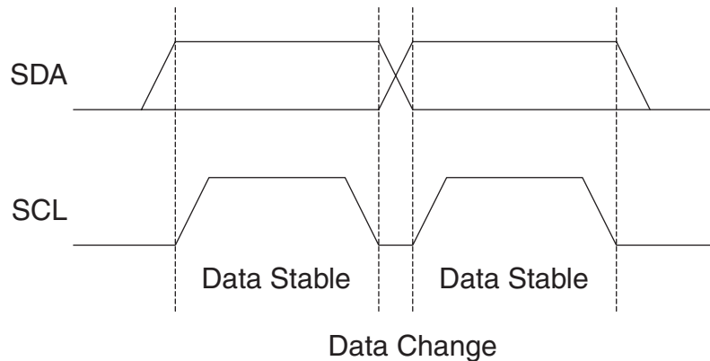
Figure 24-1. Data Validity
