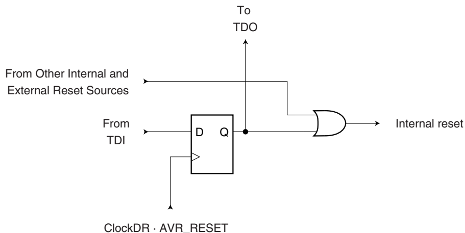
Figure 28-1. Reset Register
