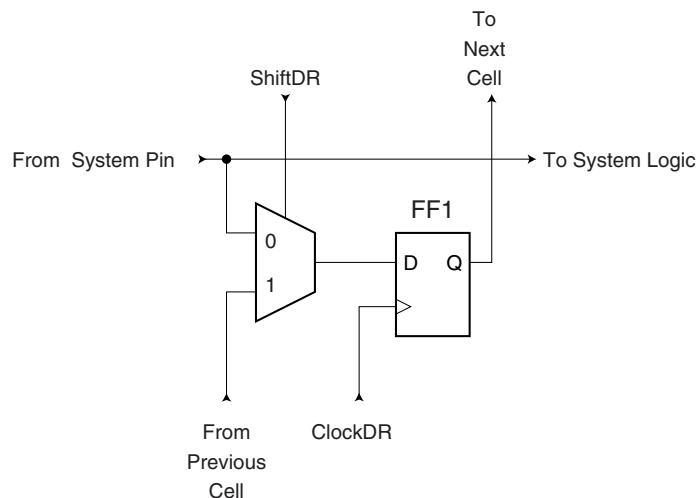
Figure 28-4. Observe-only Cell
