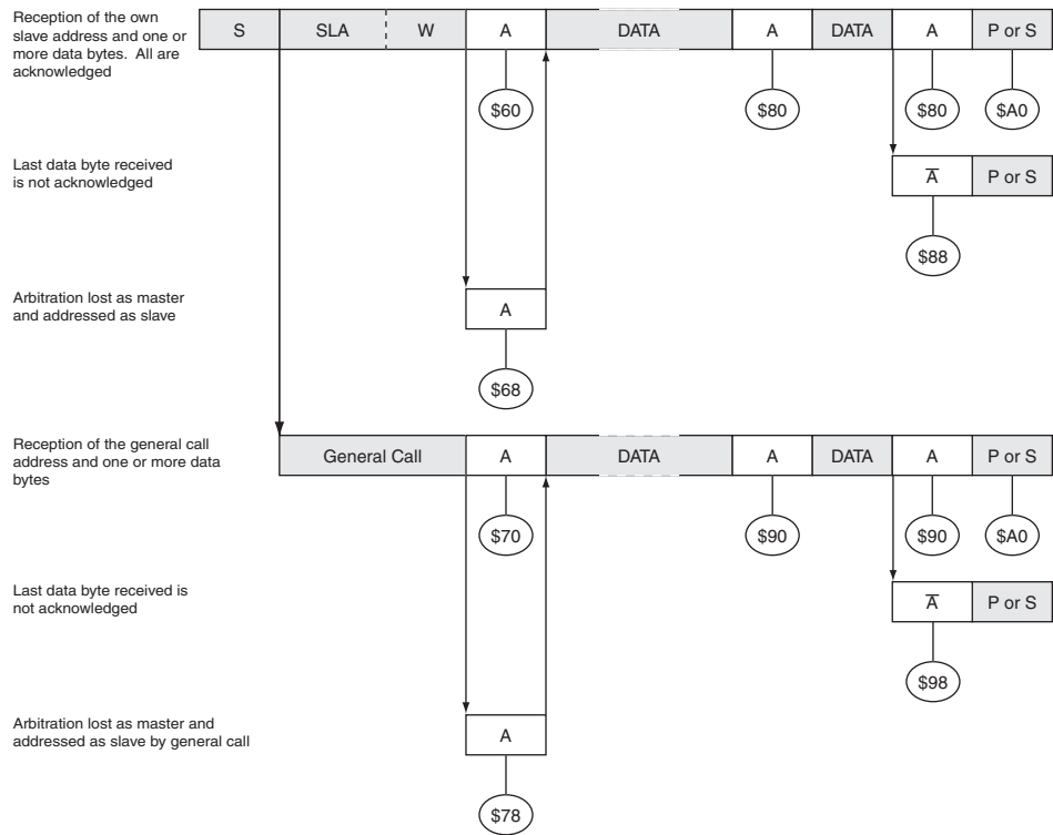
Figure 24-15. Formats and States in the Slave Receiver Mode
