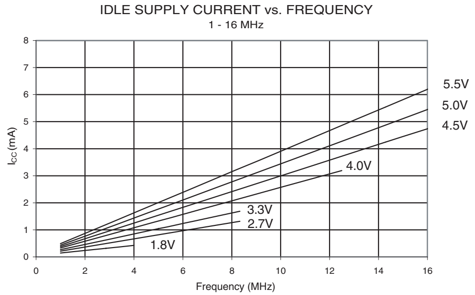
Figure 32-7. Idle Supply Current vs. Frequency (1 - 16 MHz)
