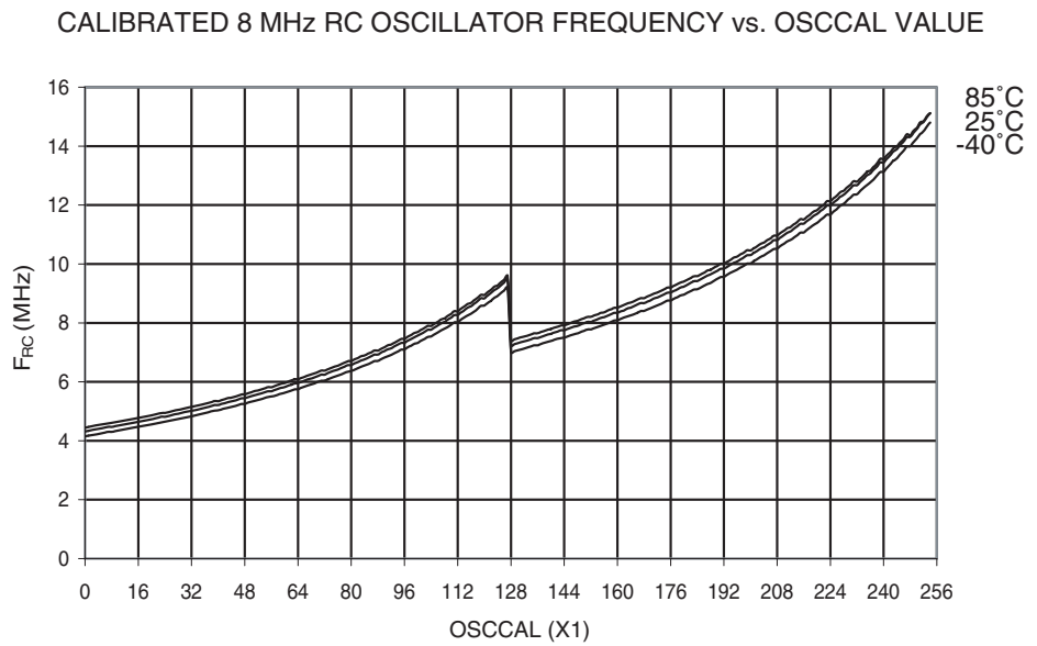
Figure 32-39. Calibrated 8 MHz RC Oscillator Frequency vs. Oscal Value
